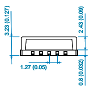
VS9000 side view
